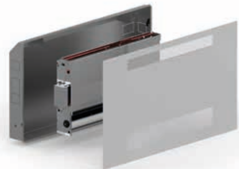
VD Vertical with CCM outer casing and MPK panel
